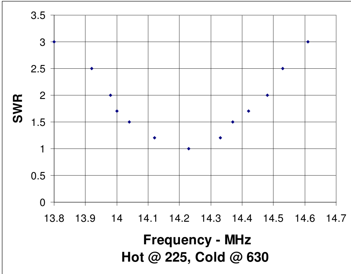
TAK-tenna 20 Bandwidth Data
